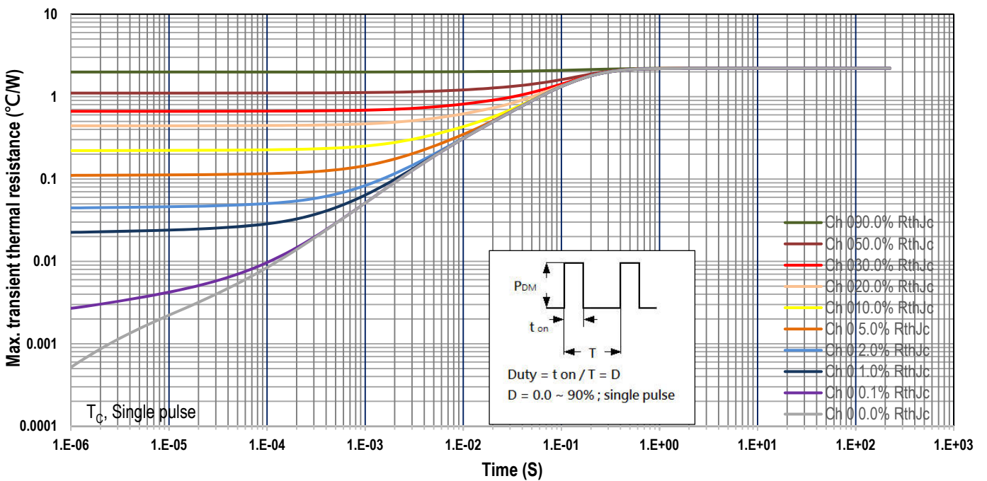
Fig.12 Transient Thermal Impedance
