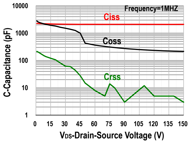
Fig. 7: Typical Capacitance Variation Vs V_{DS}
