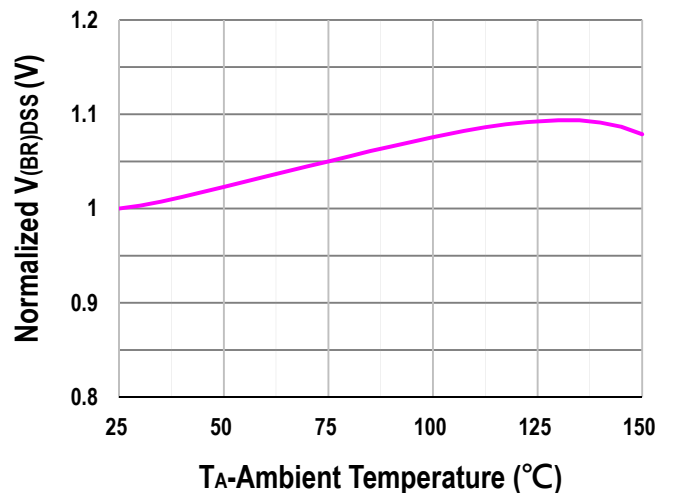
Fig. 6: Normalized V_{(BR)DSS} Voltage Vs T_A
